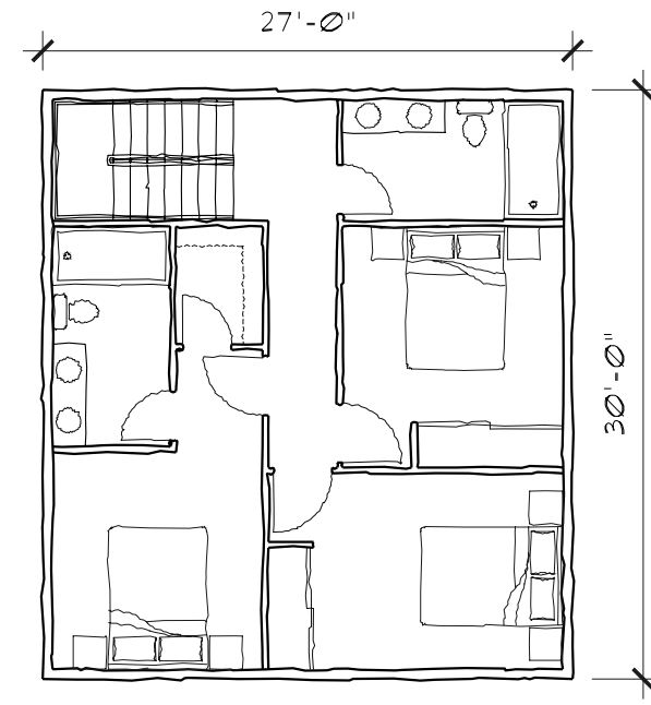
SECOND FLOOR PLAN 2
