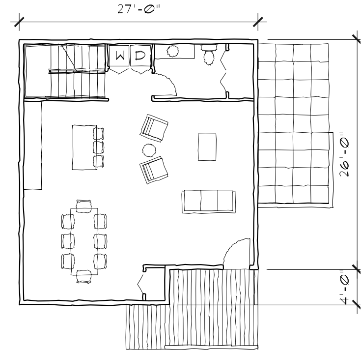
FIRST FLOOR PLAN 1
