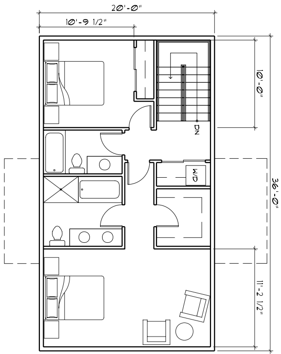
HOUSE C UPPER LEVEL PLAN 1
